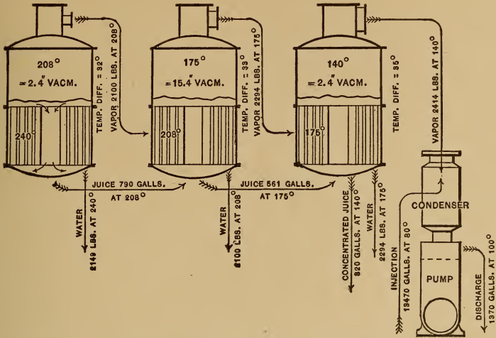
Fig. 120. TRIPLE EFFECT EVAPORATION.
